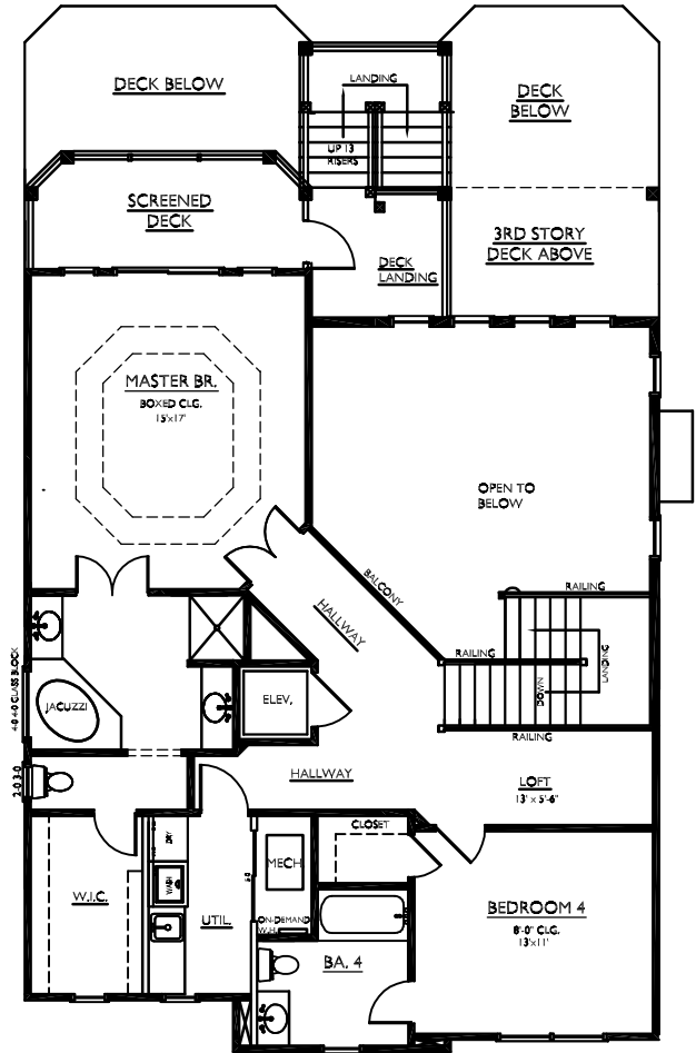
SECOND FLOOR PLAN SCALE: 1/4" = 1'-0"
